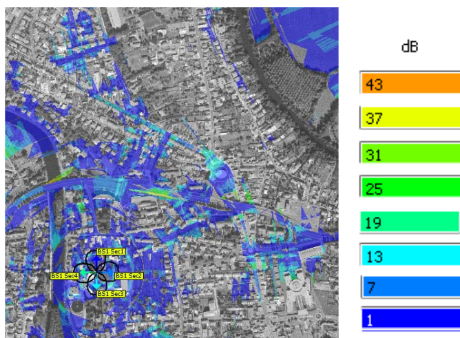
Coverage difference using 3D ray tracing or not with HR data.
