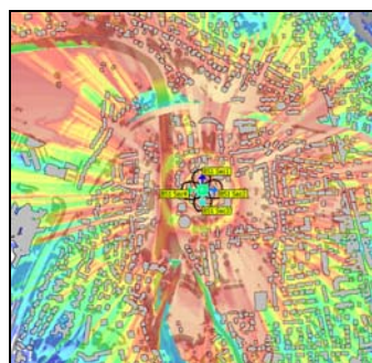
Canyon effect in High Resolution Urban environment (deterministic model)
