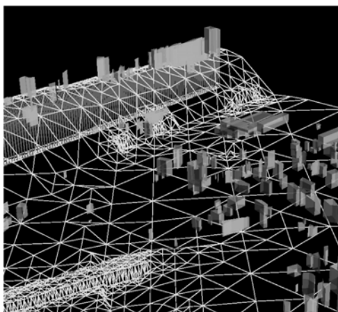
DTM in Wire frame and true-orthophoto with the blg file on top of it in ICS Telecom nG
